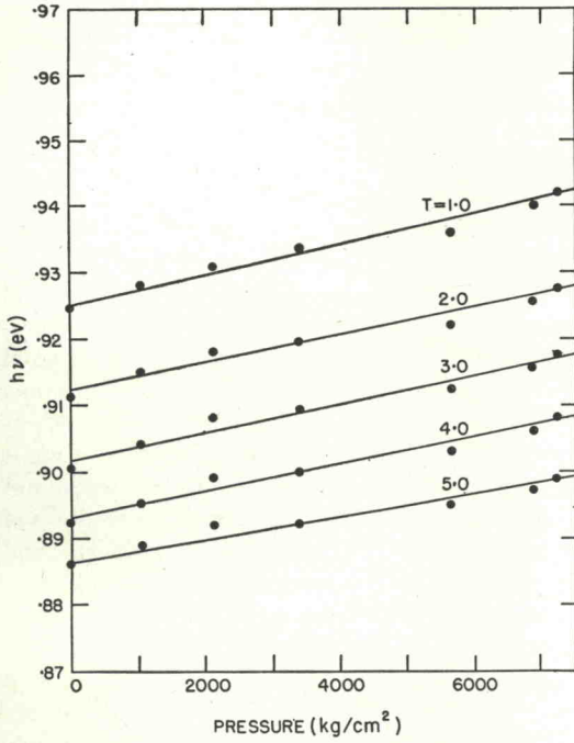
FIG. 14. Isotransmission plot of 13 per cent silicon in germanium alloy. Average slope = 2.08 \times 10^{-12} eV/dyne-cm -2 .
