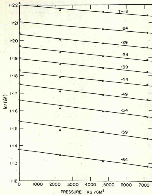
FIG. 17. Silicon isotransmission data. Average slope is -1.3 \times 10^{-12} eV/dyne \text{-cm}^{-2} .
